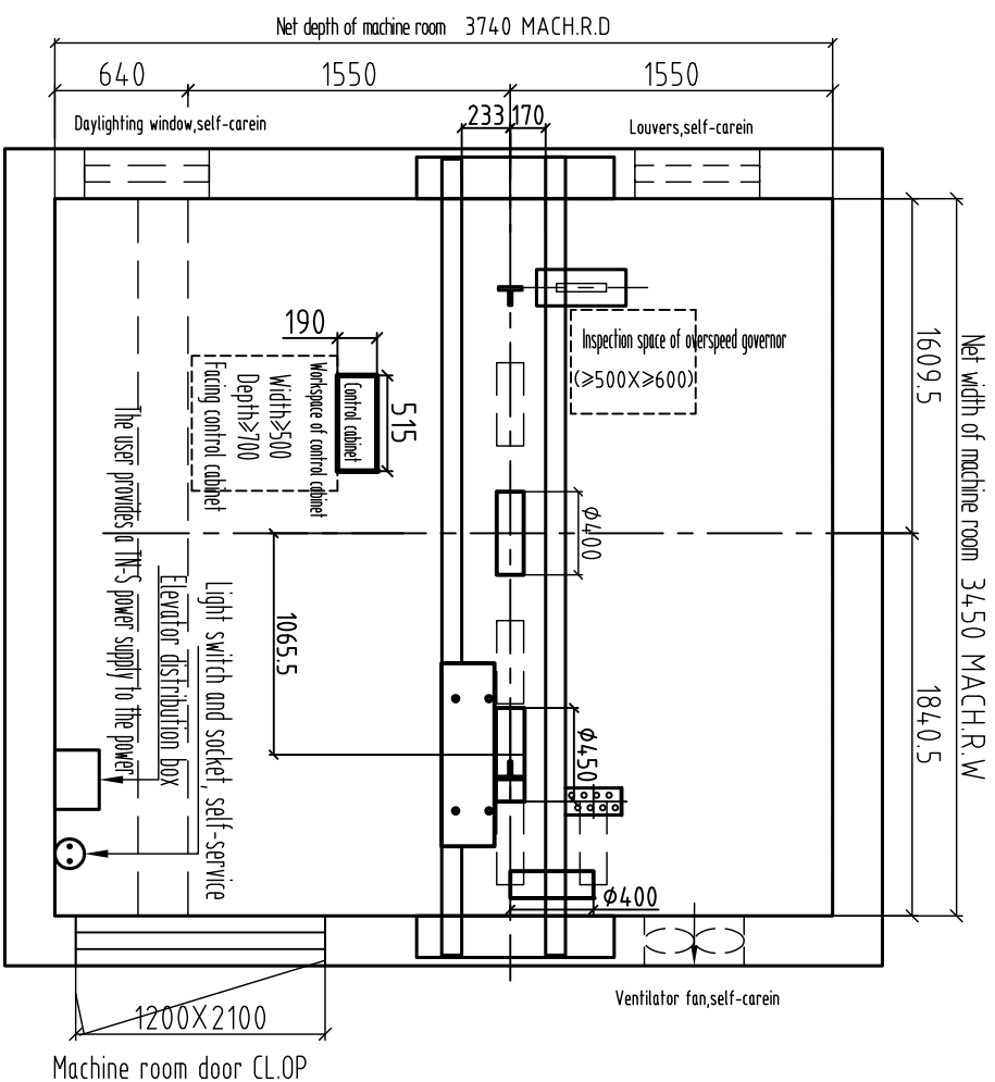
Plane figure of machine room
