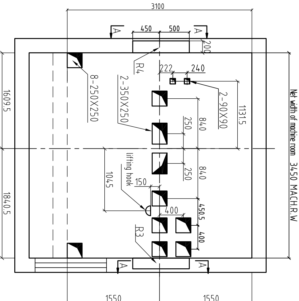
Foreseen hole diagram of machine room
