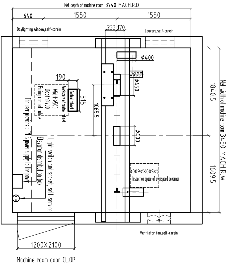
Plane figure of machine room
