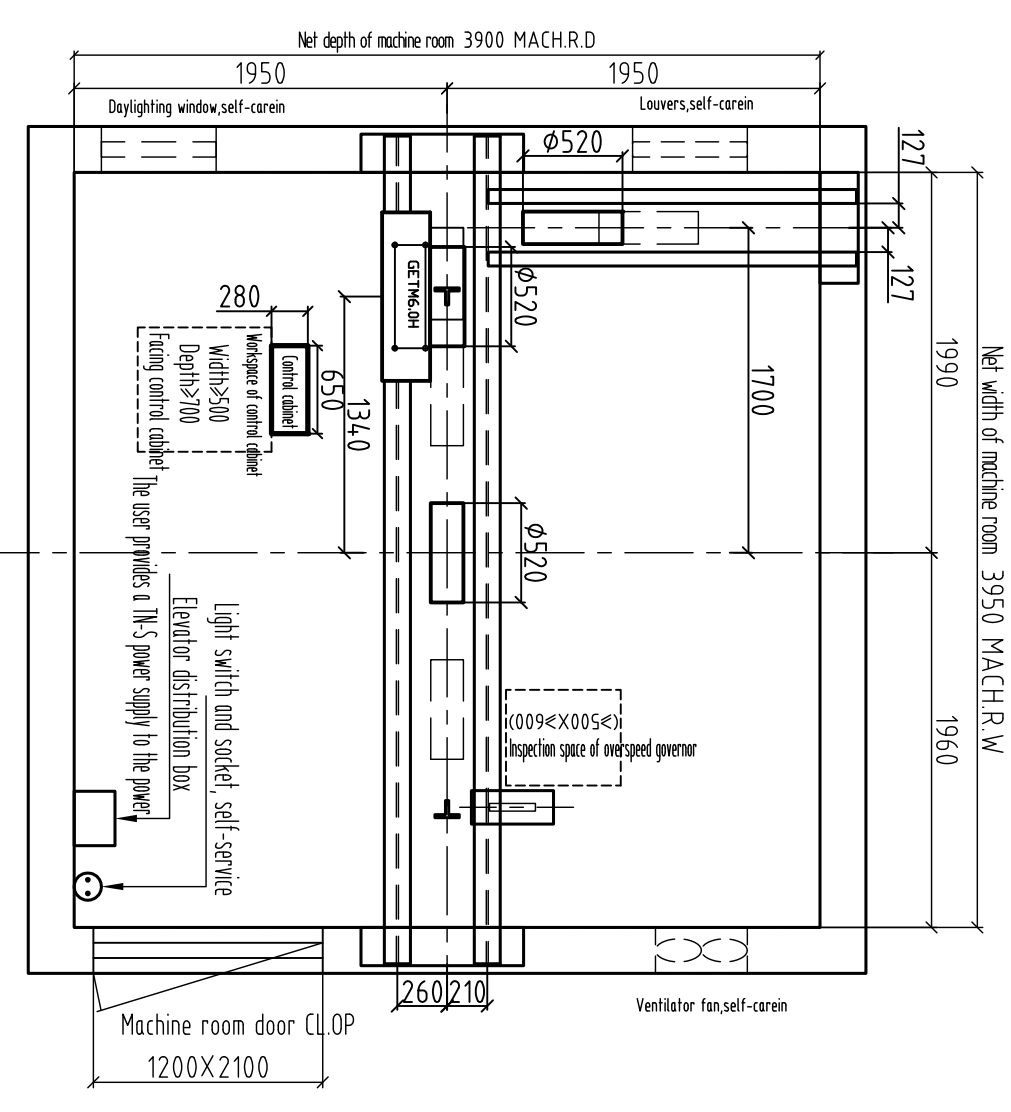
Plane figure of machine room
